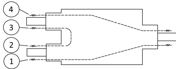
Transition unit, straight 1; 2 or 3; 4 should be looped
